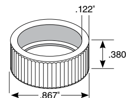
Heavy Wall Loc-Down® Bushing Part No. 11520
