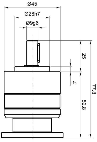
1 STAGE RATIO: 4:1 - 6:1
