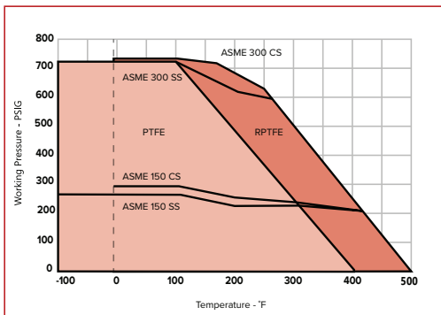
PTFE & RPTFE Seat
