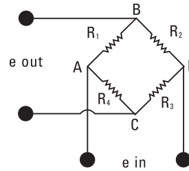
Figure 50. Wheatstone Bridge
