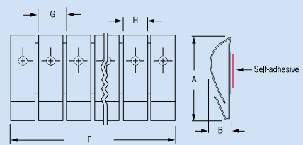
Stick on 2303
