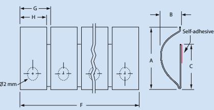
Stick on 2363
