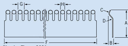
Circular Finger 2601
