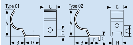
Angle Fingerparts 2505 (short pieces)
