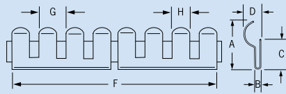
Clip on 2105
