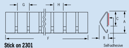
Stick on 2301
