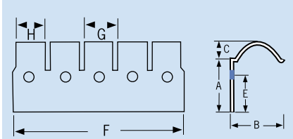
Angle Fingerstrips 2501
