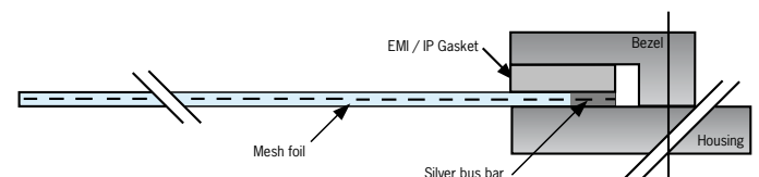
Standard mesh foil mounted by a clamping construction with an EMI gasket. A water seal is optional.
