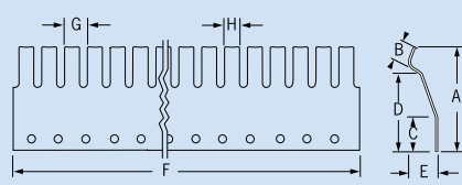
Contact Finger 2705
