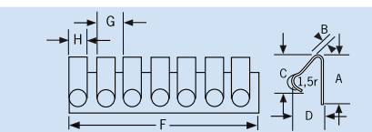
Circular Finger 2605
