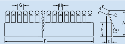
Circular Finger 2602
