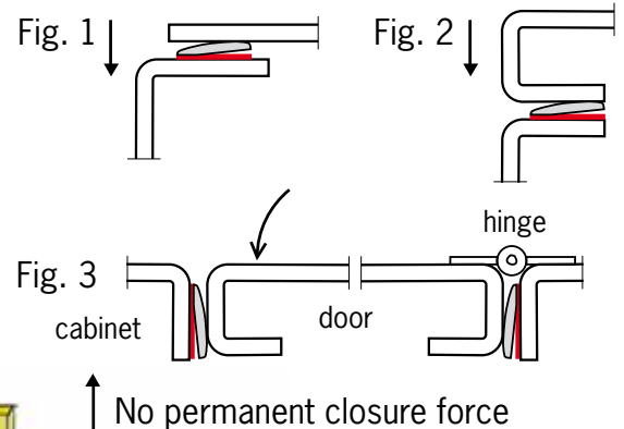
For doors: gaskets with low closure force, to prevent bending of doors, lids and panels
