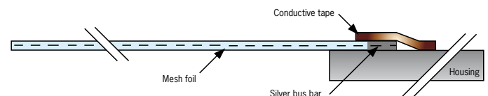
Standard mesh foil mounted with conductive tape 3201
