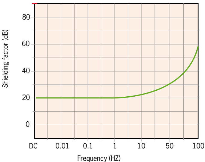
Shielding performance 2 mm Mu-ferro-HD
