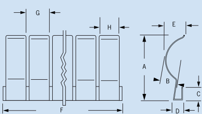
Clip on 2103
