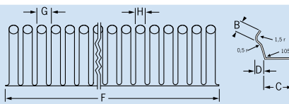
Circular Finger 2603
