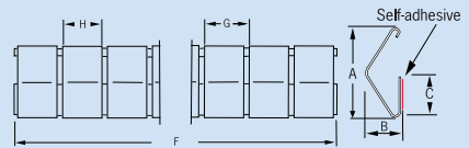
Stick on 2334
