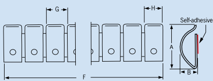
Stick on 2365
