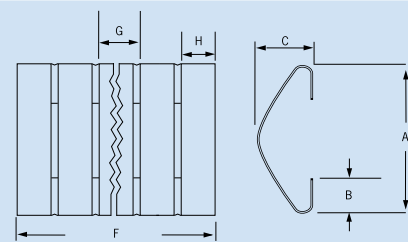
Snap on 2203
