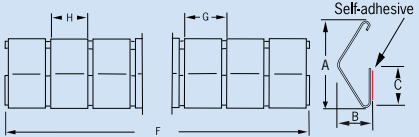
Stick on 2364
