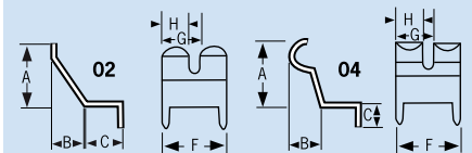
Angle Fingerparts 2504 (short pieces)
