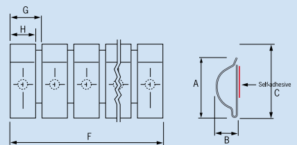
Stick on 2302
