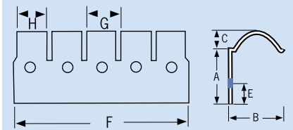
Angle Fingerstrips 2502
