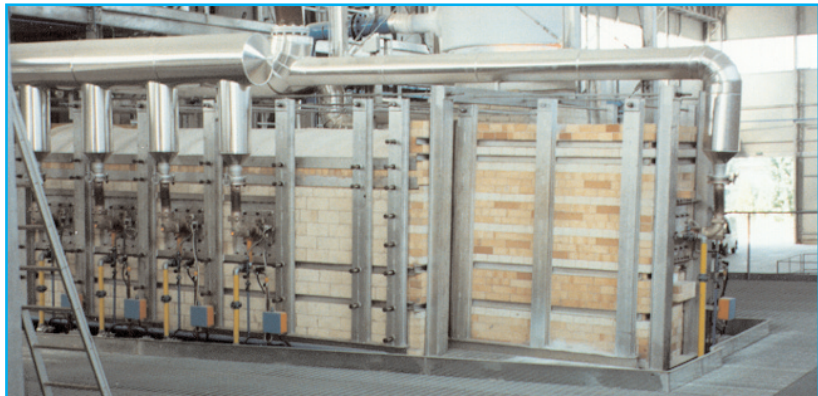
Rocking frit melting furnace for pre-heated air (450° C), "Nozzle Mix" burners (Poppi Eurotech)
