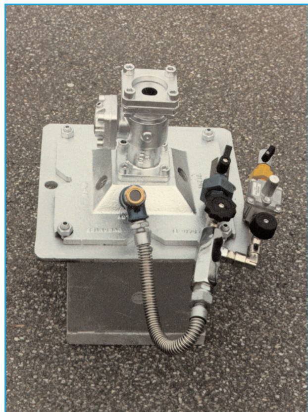
Pre-assembled "Nozzle Mix" burner (Ferré c/o Ilva)
