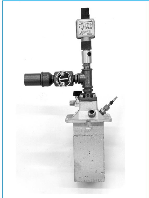
Pre-assembled "Nozzle Mix" burner groups (Intercer)
