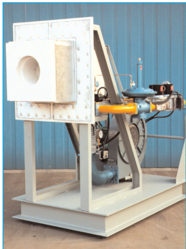
Pre-assembled group on movable cart with "Nozzle Mix" burner for furnace pre-heating (L.A.G. Laminati Alluminio Gallarate)
