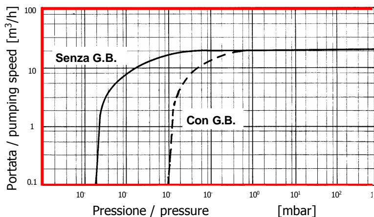
Curve di portata – Pumping speed curves
