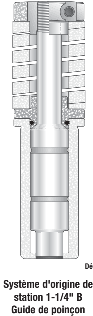
Station 1-1/4" B type d'origine
