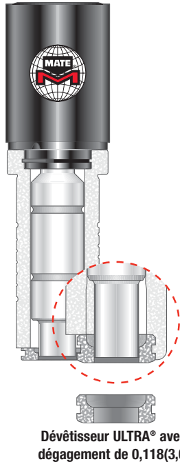
Station 1-1/4" B ULTRA®
