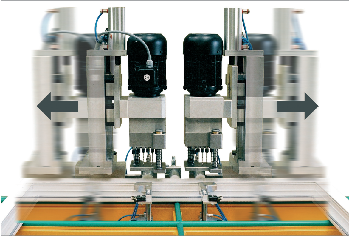
Drilling unit with fixed or automatically pivoting six-spindle drilling head and spring-loaded drill spectacles.
