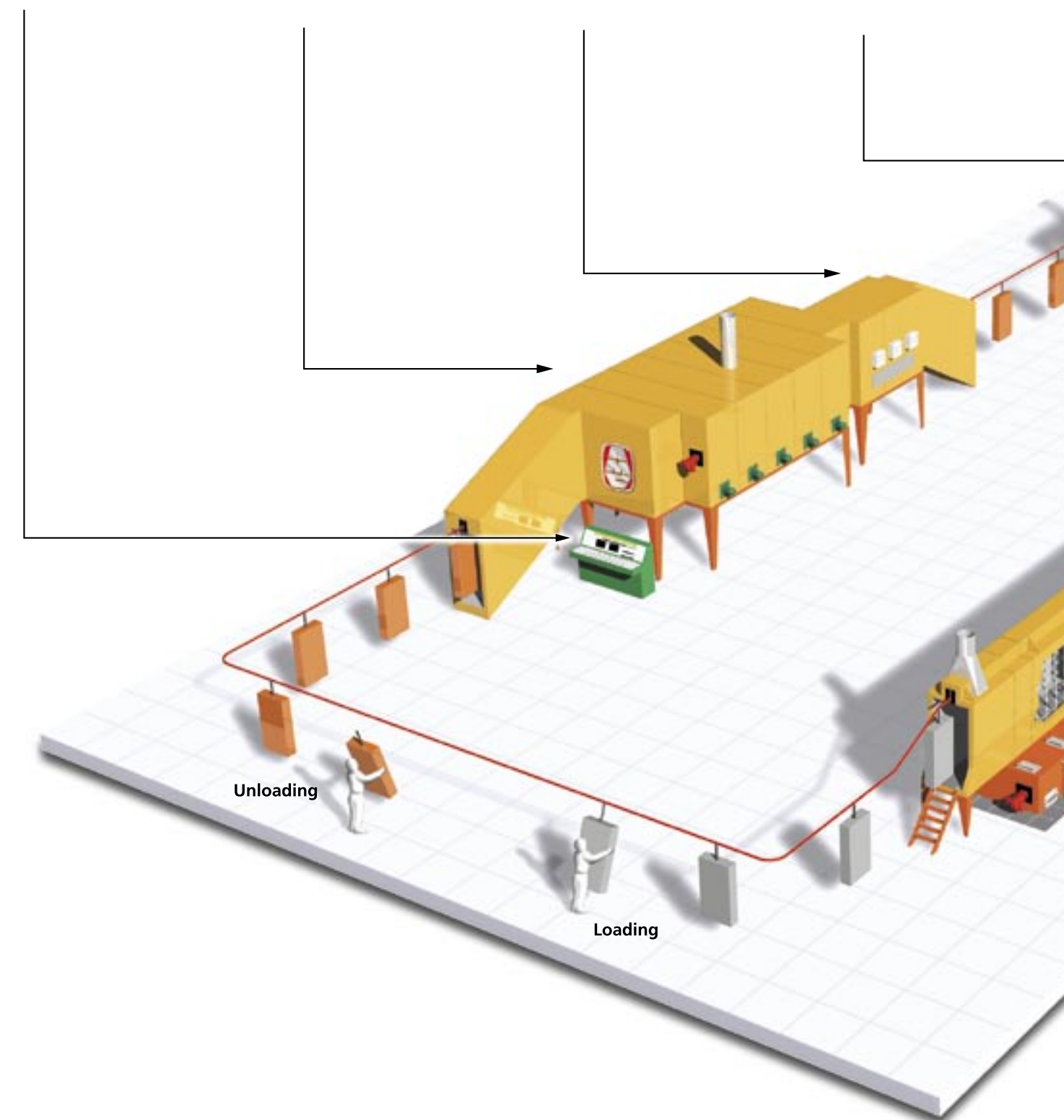
AMC Electric panel control Ets NORPLAST Convection cure oven with floor ducting Ets PEL JOB Infra-red curing oven with gas fired radiant emitters Ets BAYARD Spray booth with built-in cartridge filters
