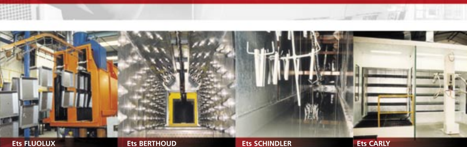
Ets FLUOLUX Pretreatment tunnel Ets BERTHOUD Drying tunnel after pretreatment Ets SCHINDLER Dip-coating paint tank Ets CARLY Spray booth
