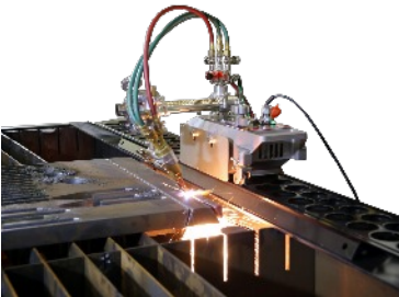
IK-12 MAX3/1 Torch
