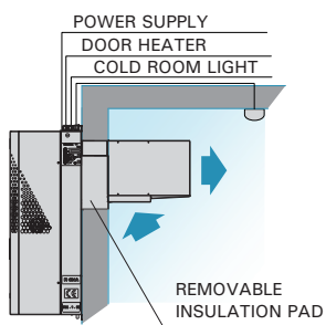
Plug-in mounting
