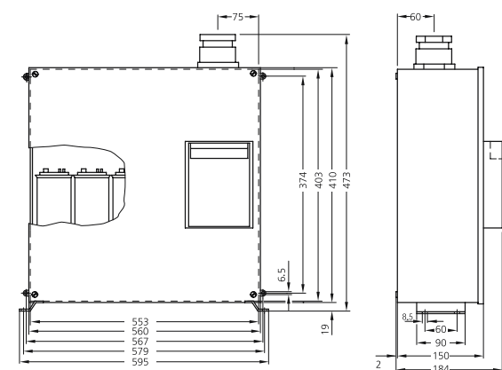
Dimensional drawing LKSLT Case type 2 (50 to 60 kvar)
