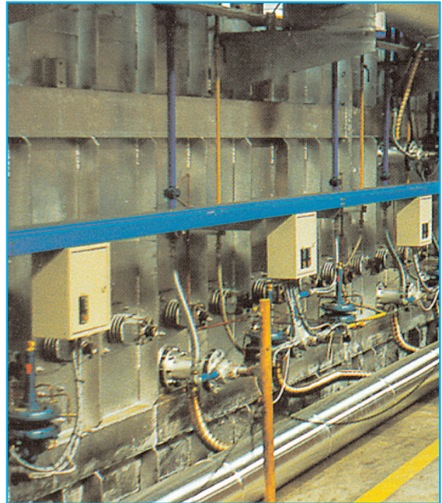
Heat treat furnace for strips with recuperative, radiant burners, model SER (Falck)
