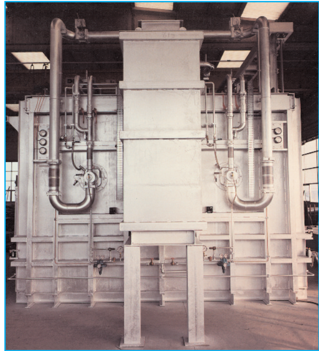
Aluminium holding furnaces with dual fuel burners (gas/L.P.) (Continuous)
