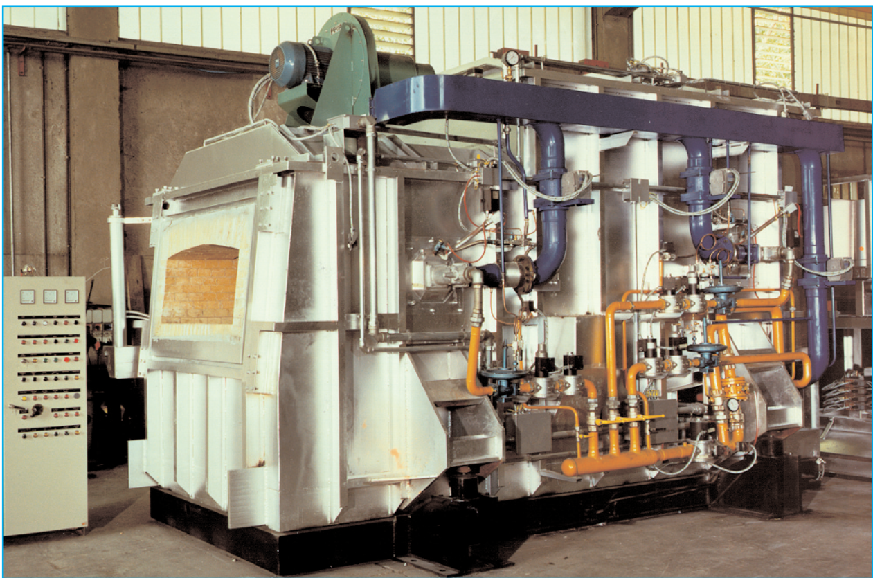
Melting furnace and aluminium holding furnace with "Nozzle Mix" burners
