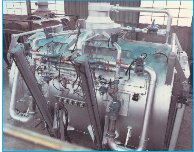
Aluminium holding furnaces with dual fuel burners (gas/L.P.) (Continuous)
