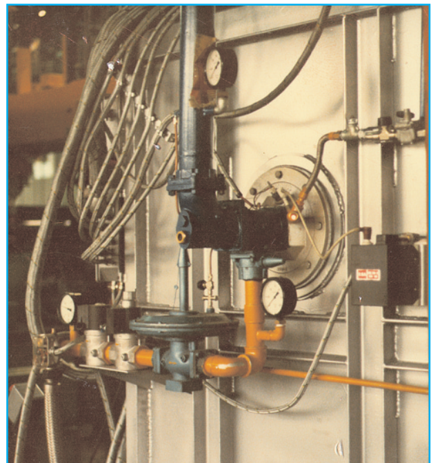
Detail of "Nozzle Mix" burner for melting and aluminium holding furnaces
