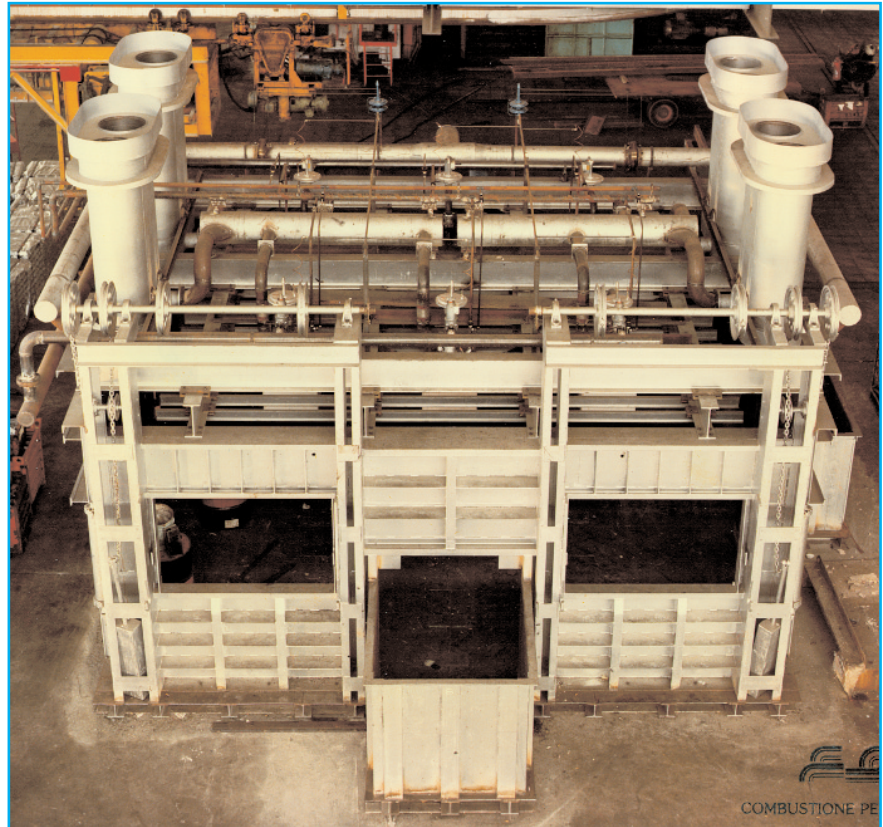
Melting furnace and aluminium holding furnace with radiant burners (roof suspension) (Alutek)
