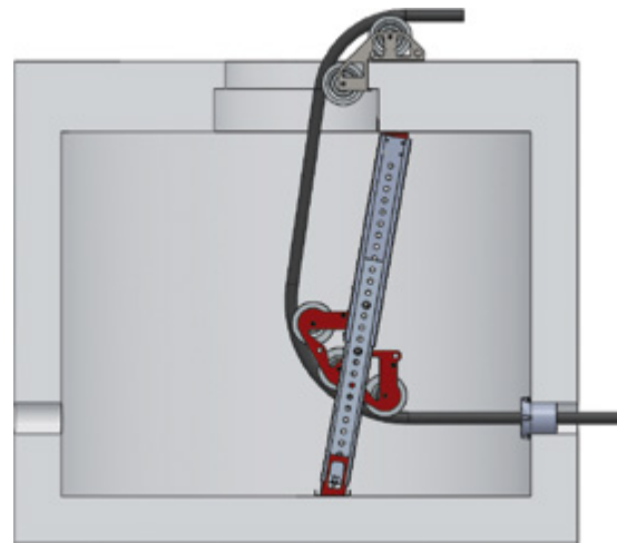
Full Assembly
