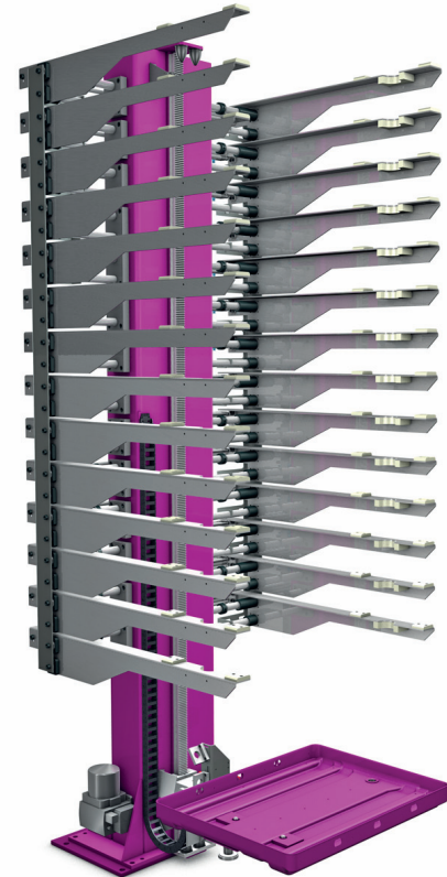
Lifting column 2 | System for intermediate stacking with additional features such as central lubrication and auxiliary guides.
