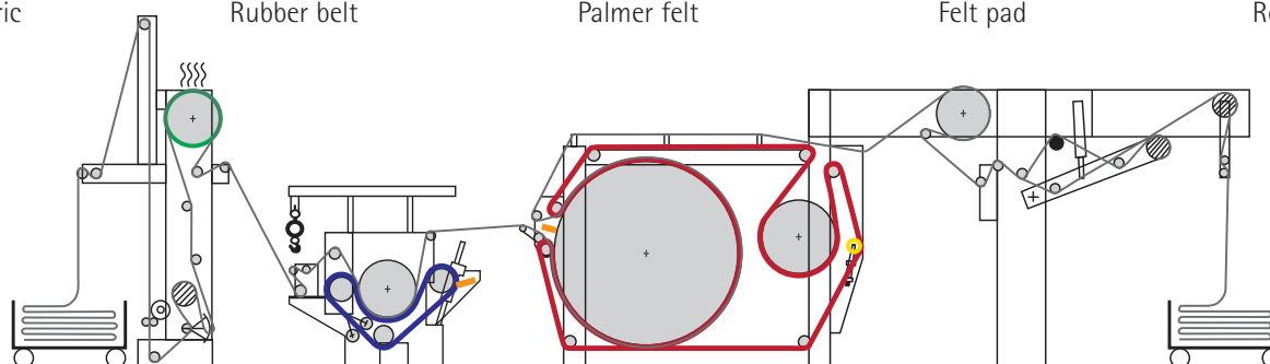
Rubber belt
