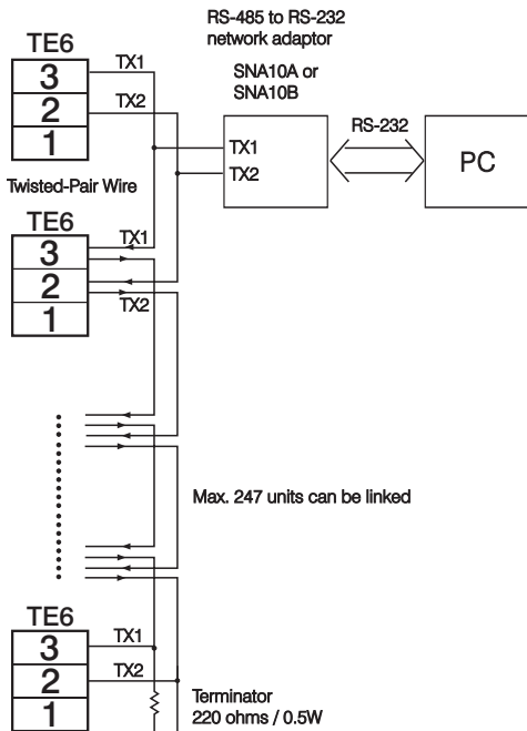
Figure 2.21 RS-485 Wiring
