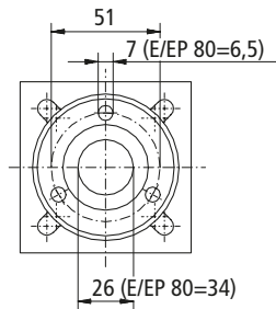
Raccordement EHL
