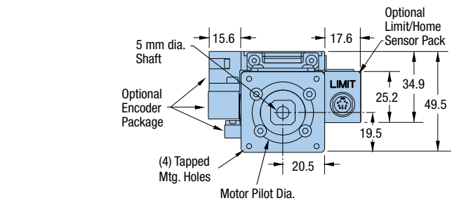
Enlarged End View (with Encoder and Limit/Home Sensor Pack Option)
