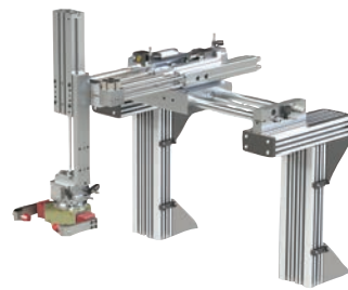
DIRECTCONNECT™ Pick-and-Place Module
